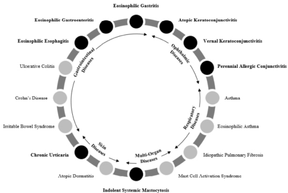
Figure 1. Select Eosinophil and Mast Cell Related Diseases
